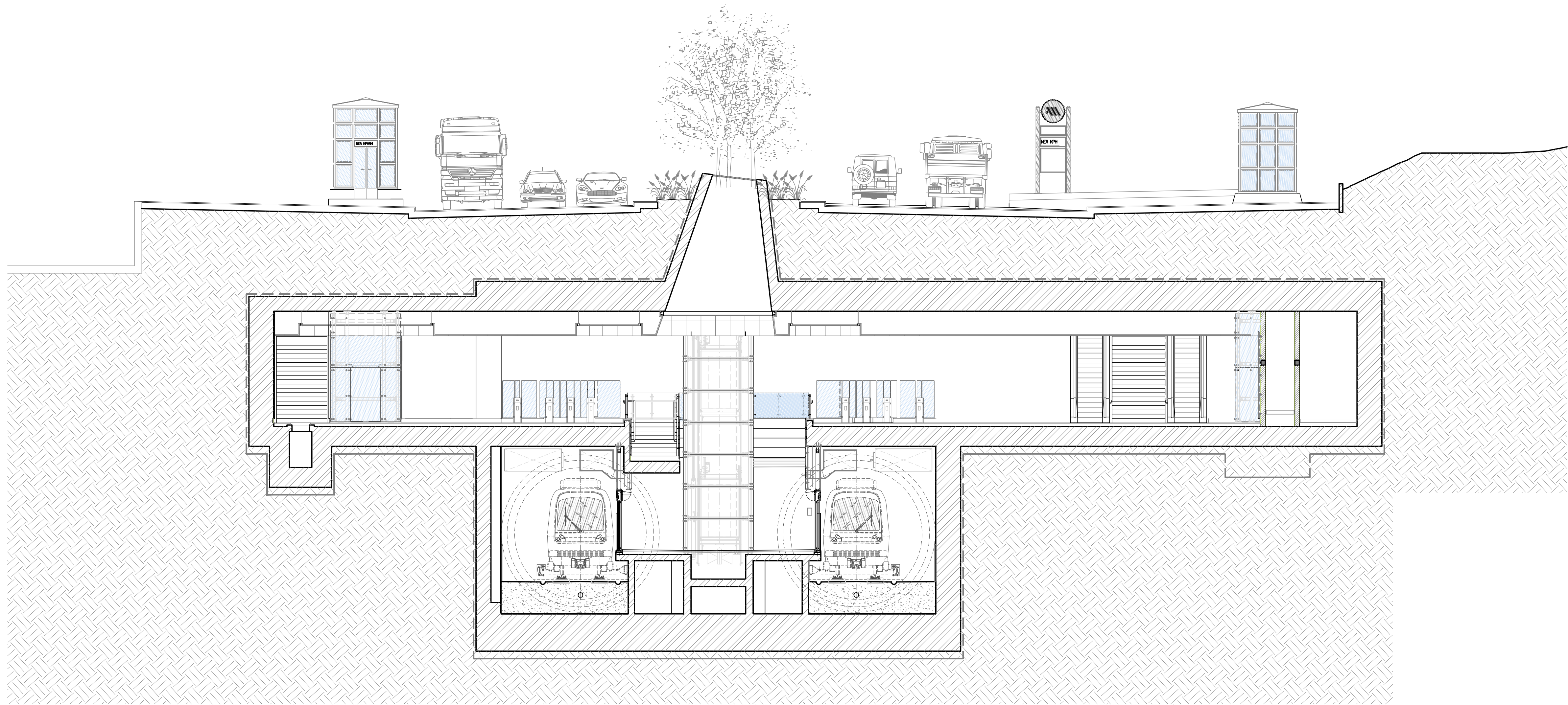
TOMH-04H B-B SECTION/ELEVATION B-B
